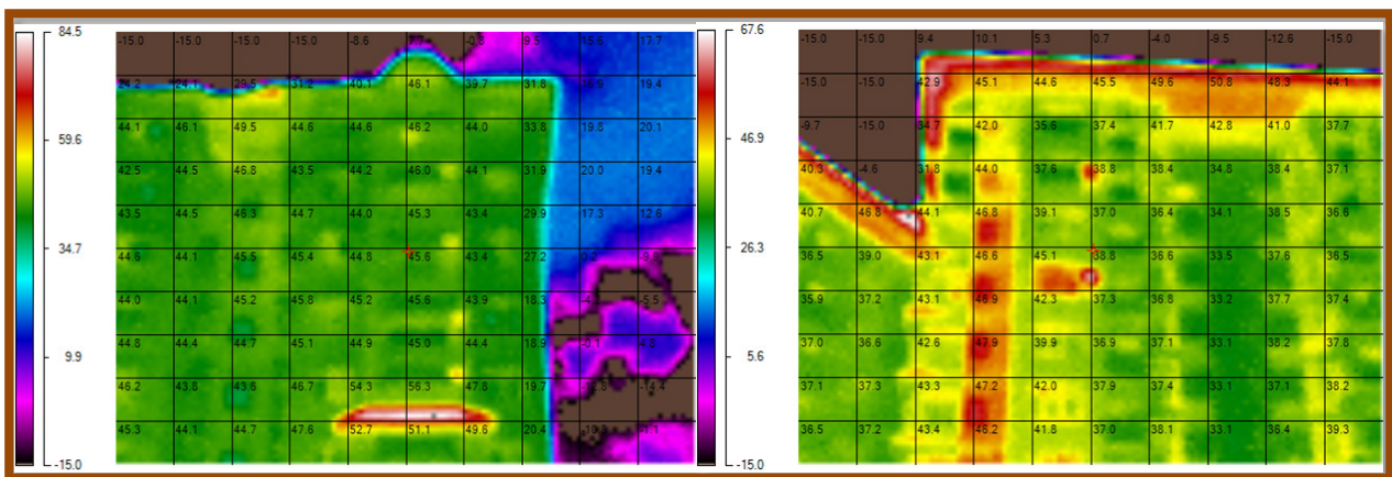
Figure 8: Thermal images for both case studies colonial style (left) and vernacular style (right) at 2:00 pm
