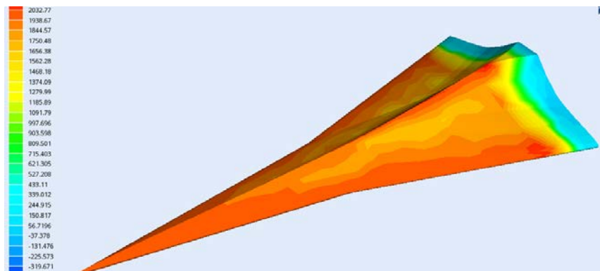
Figure 2: Distribution of heat flows on the surface of the winged vehicle at M_\infty = 17 . In red - temperature of 1939 K
