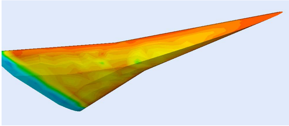
Figure 4: Distribution of heat flows on the surface of the winged vehicle at M_\infty = 17 .
