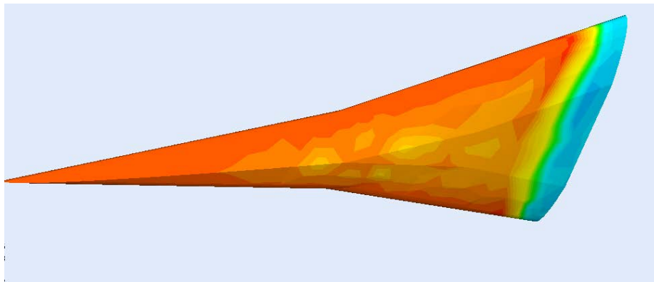
Figure 5: Distribution of heat flows on the surface of the winged vehicle at M_\infty = 17 .
