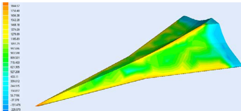
Figure 1: Distribution of heat flows on the surface of the winged vehicle at M_\infty = 17 . Non-catalytic surface. In a yellow - temperature of 1278 K.
