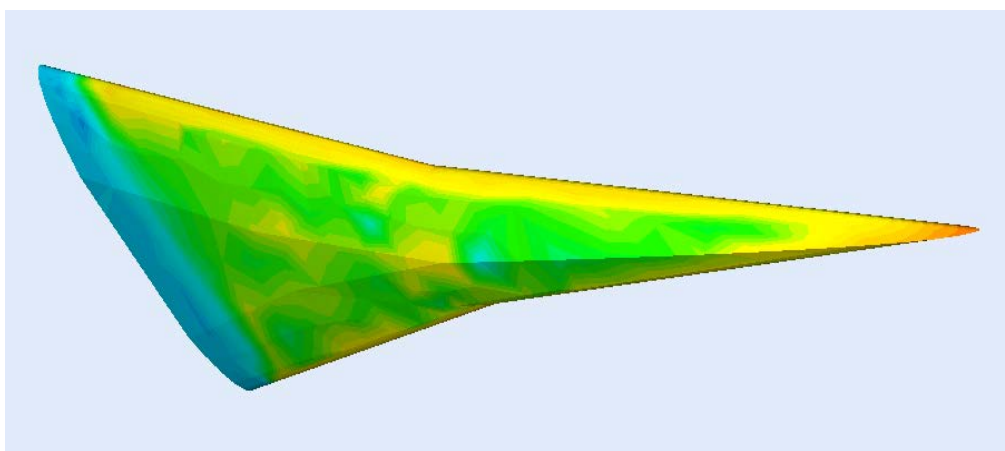
Figure 3: Distribution of heat flows on the surface of the winged vehicle at M_\infty = 17 . Non-catalytic surface. In a yellow - temperature of 1278 K
