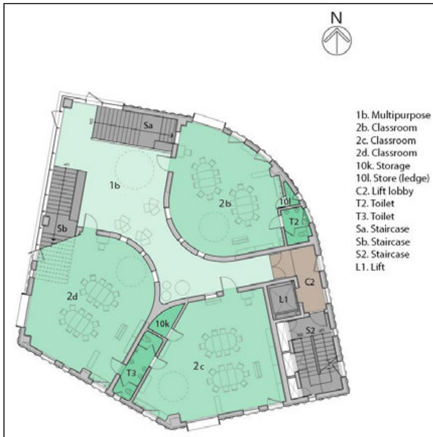
Figure 3: First Floor Plan
