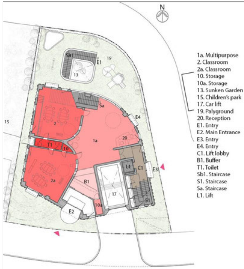
Figure 1: Site Plan and Ground Floor Plan
