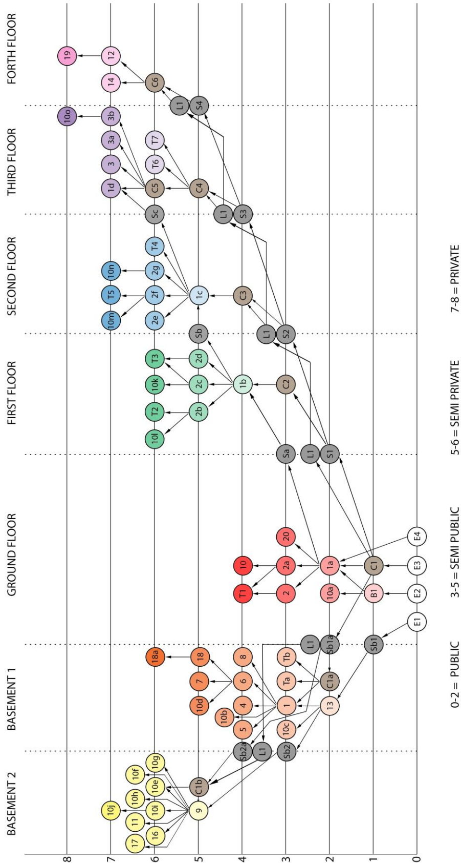
Figure 7: Overall Justified Graph of Flower Kindergarten.
