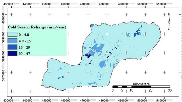
Figure 10: Simulated yearly recharge in the cold season
