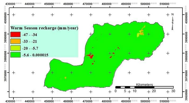
Figure 11: Simulated yearly recharge in the warm season
