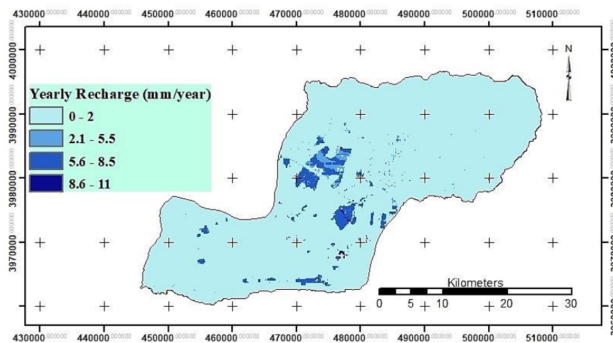
Figure 9: Simulated yearly recharge map
