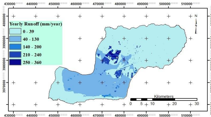
Figure 6: Simulated surface runoff map
