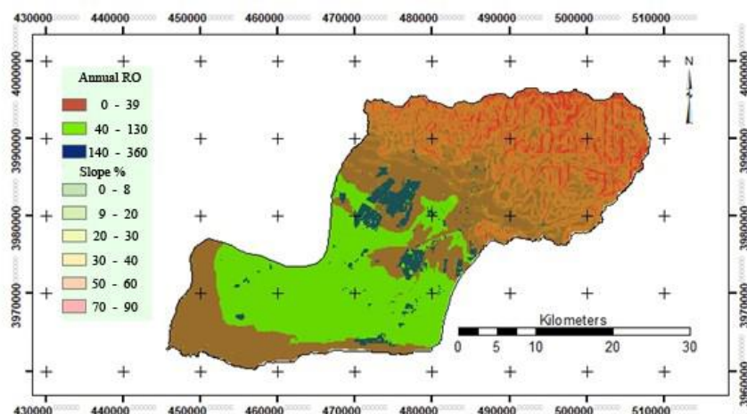
Figure 7: Simulated surface runoff map in different slopes
