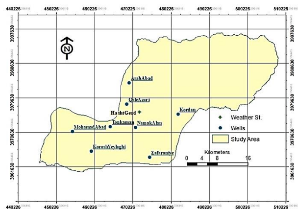
Figure 2: Location of selected wells and the Hashtgerd synoptic station
