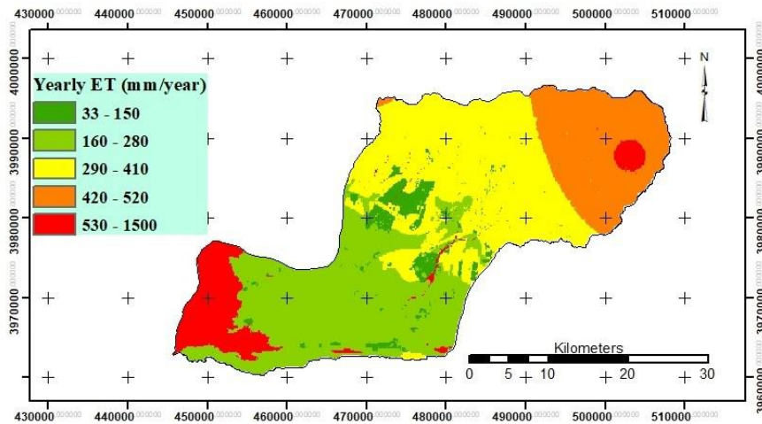
Figure 8: Simulated evapotranspiration map.
