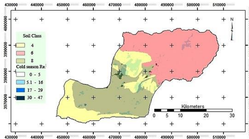
Figure 12: Simulated recharge in cold season at different soil classes
