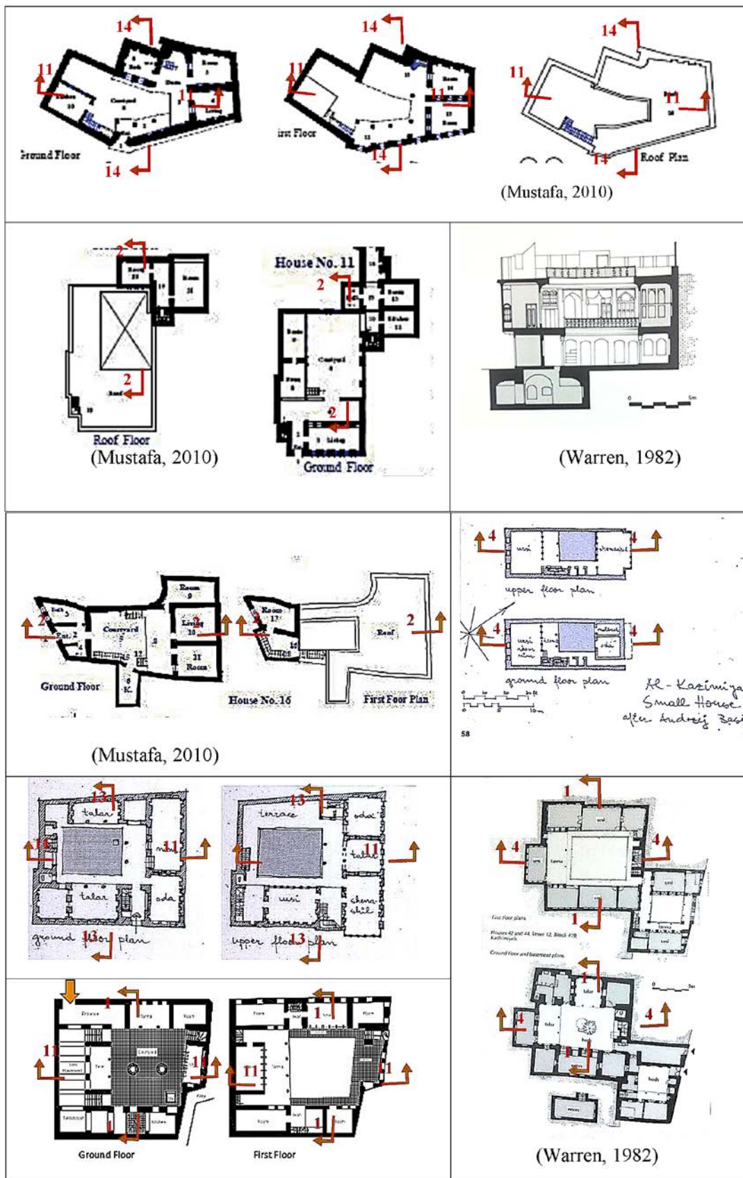
Figure 10: Floor plans of existing houses with Cy forms resembling the explored ones
