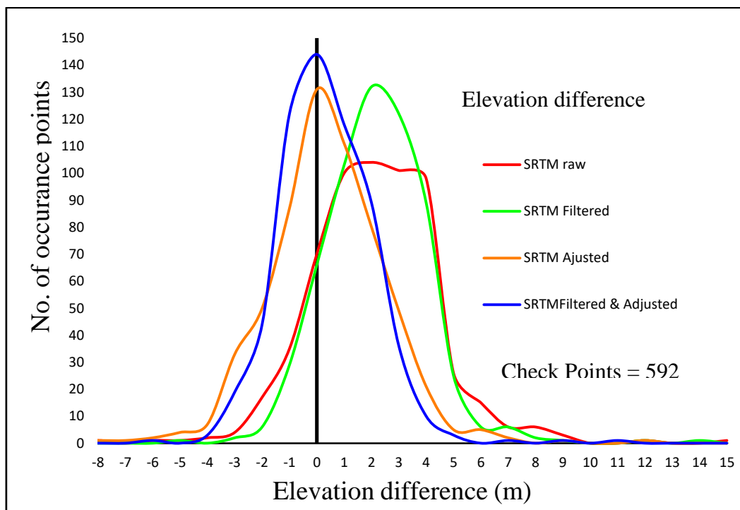
Figure 8: The histograms of elevation differences of the final accuracy assessment
