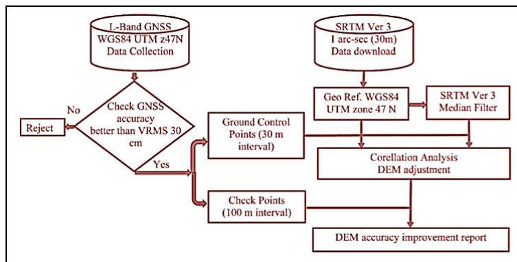
Figure 3: Methodology for SRTM Ver.3 and GNSS Data Processing and Analysis
