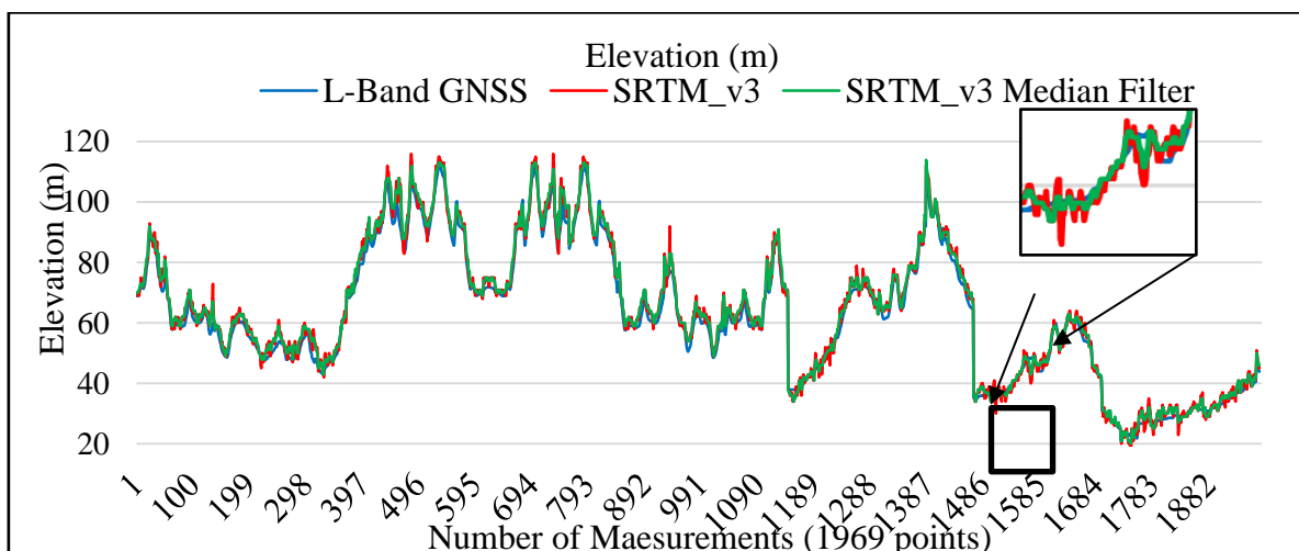
Figure 5: The difference between GNSS trajectory, SRTM raw data, and median filtered data
