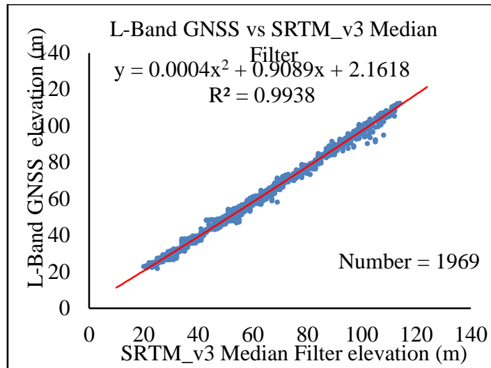
Figure 7: Vertical comparison between GNSS data with SRTM, applied with a median filter.
