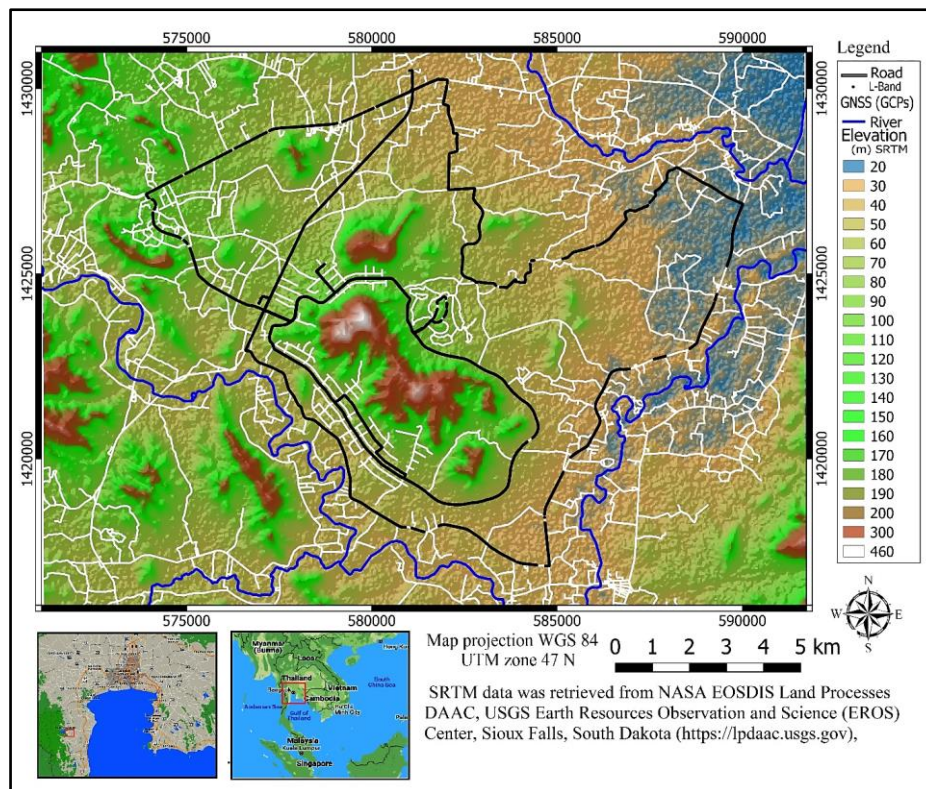
Figure 1: Topographic map of the study area with L-Band GNSS data collection points. (Courtesy of USGS EROS/NASA EOSDIS)
