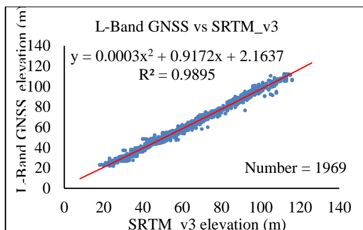
Figure 6: Vertical comparison between GNSS data with SRTM
