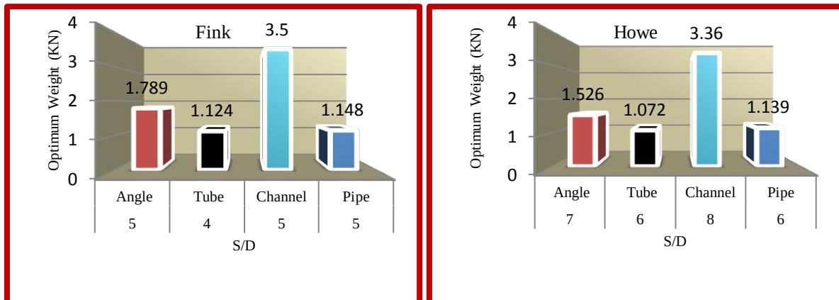
Figure 6: Optimum Fink and Howe truss weights among different cross sections under optimum S/D.
