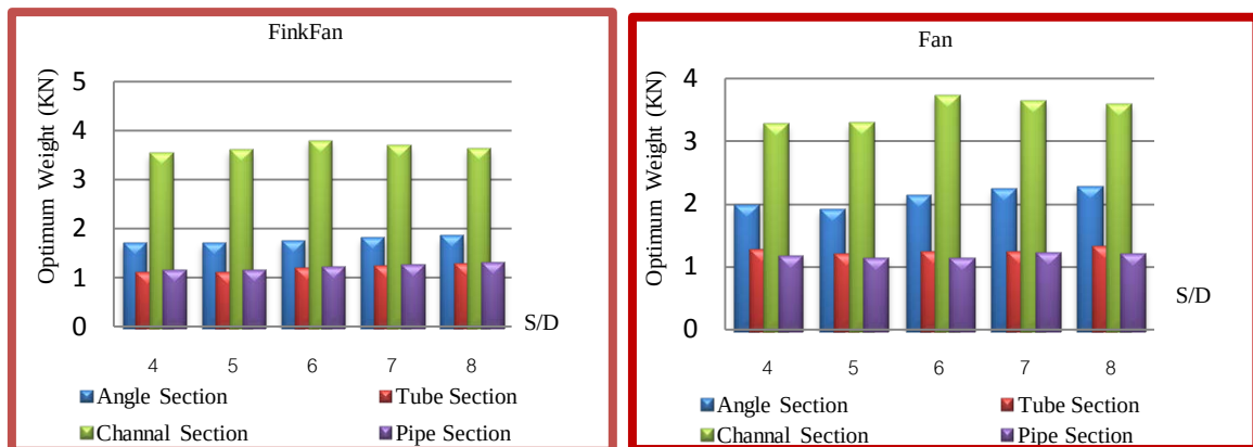
Figure 2: Optimum Fink fan and Fan Truss Weights among Different Cross Sections under Various S/D.
