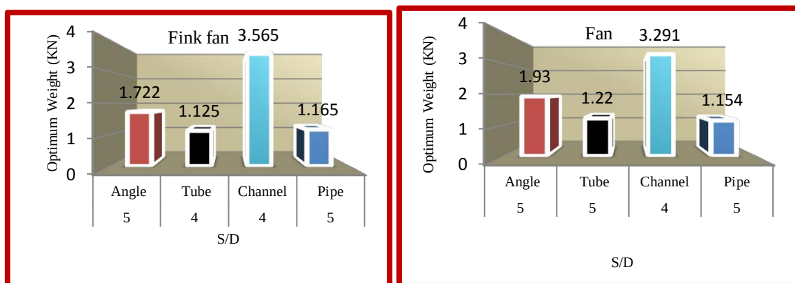
Figure 5: Optimum Fink fan and Fan Truss weights among different cross sections under optimum S/D.
