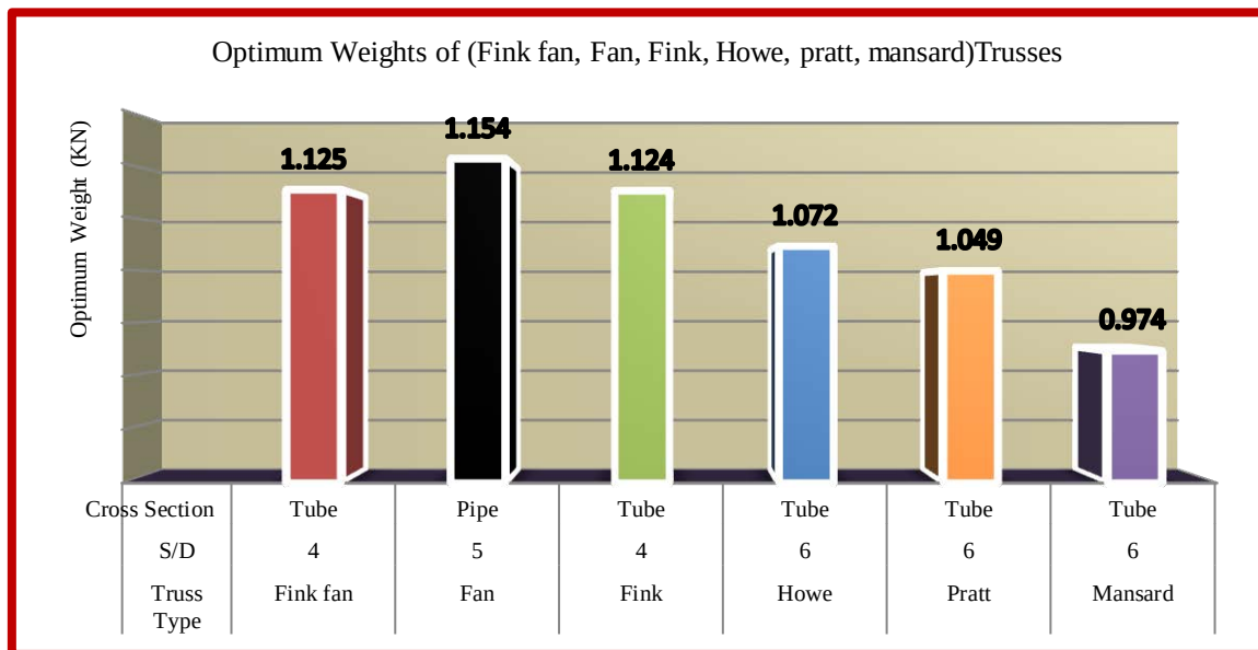
Figure 8: Optimum Weights of various Truss Types among Best Cross Sections and S/D.
