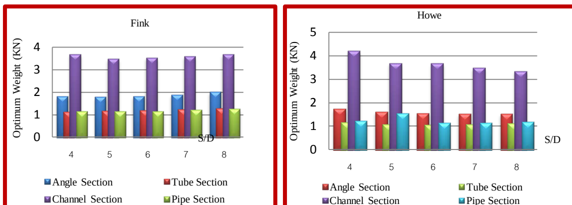
Figure 3: Optimum Fink and How Truss Weights among Different Cross Sections under Various S/D.
