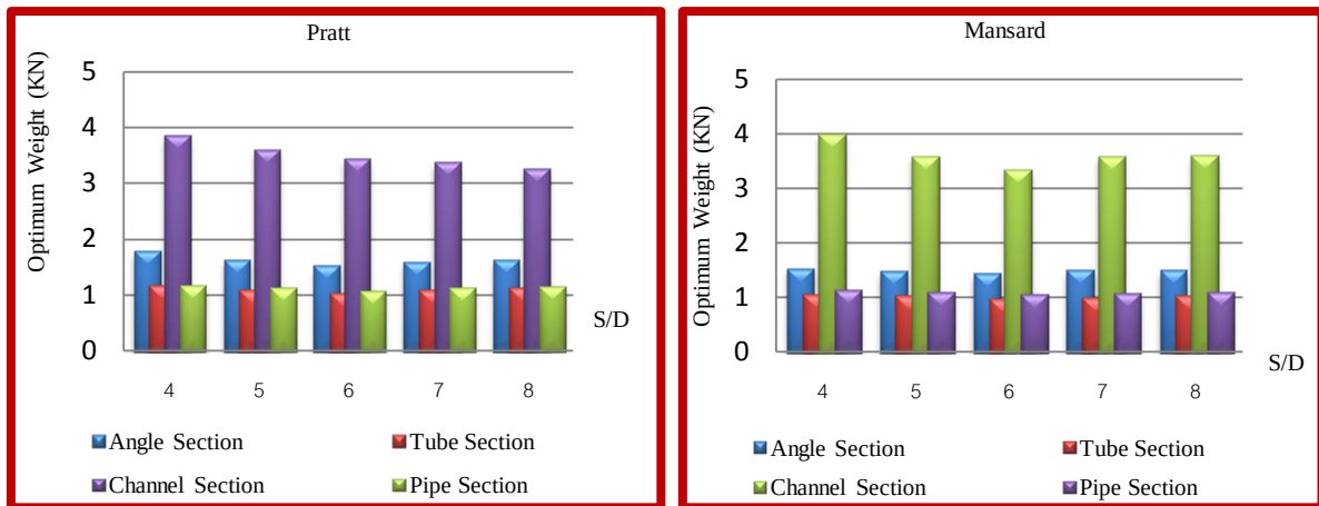
Figure 4: Optimum Pratt and Mansard Truss Weights among Different Cross Sections under Various S/D.
