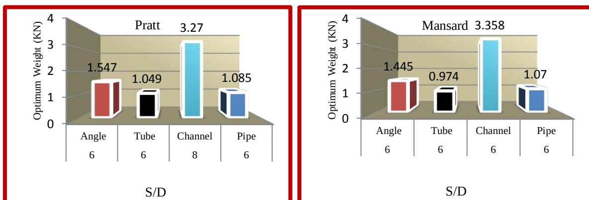
Figure 7: Optimum Pratt and Mansard truss weights among different cross sections under optimum S/D.
