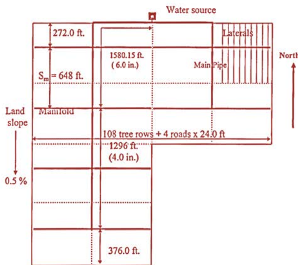
Figure 6a: Model design for farm layout and main pipe network (laterals are 16 mm PE, manifolds are SDR 26 PVC, and main lines are SDR 41 PVC).
