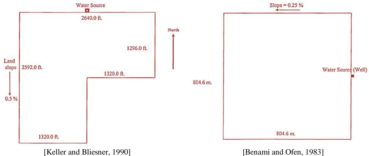
Figure 5: Orchard Field for Point-Source Drip Irrigation System.
