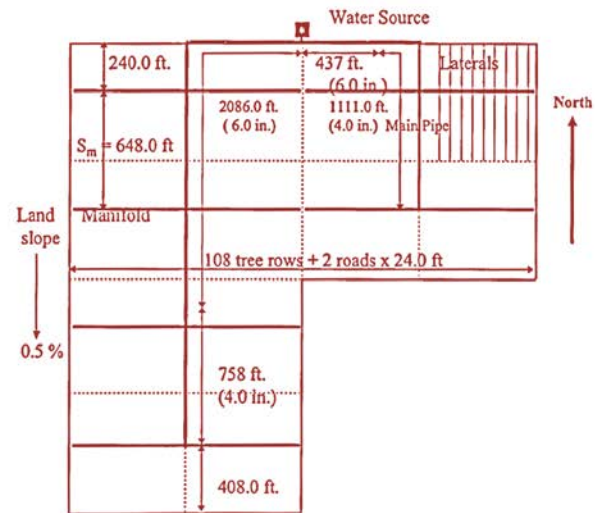
Figure 6b: Keller and Bliesner design for farm layout and main pipe network (laterals are 0.58-inch PE, manifolds are SDR 26 PVC, and main lines are SDR 41 PVC).
