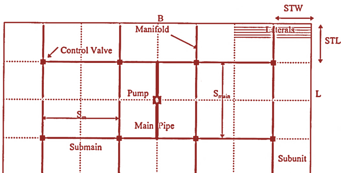
Figure 1: Configuration [1] for Trickle Irrigation Systems.
