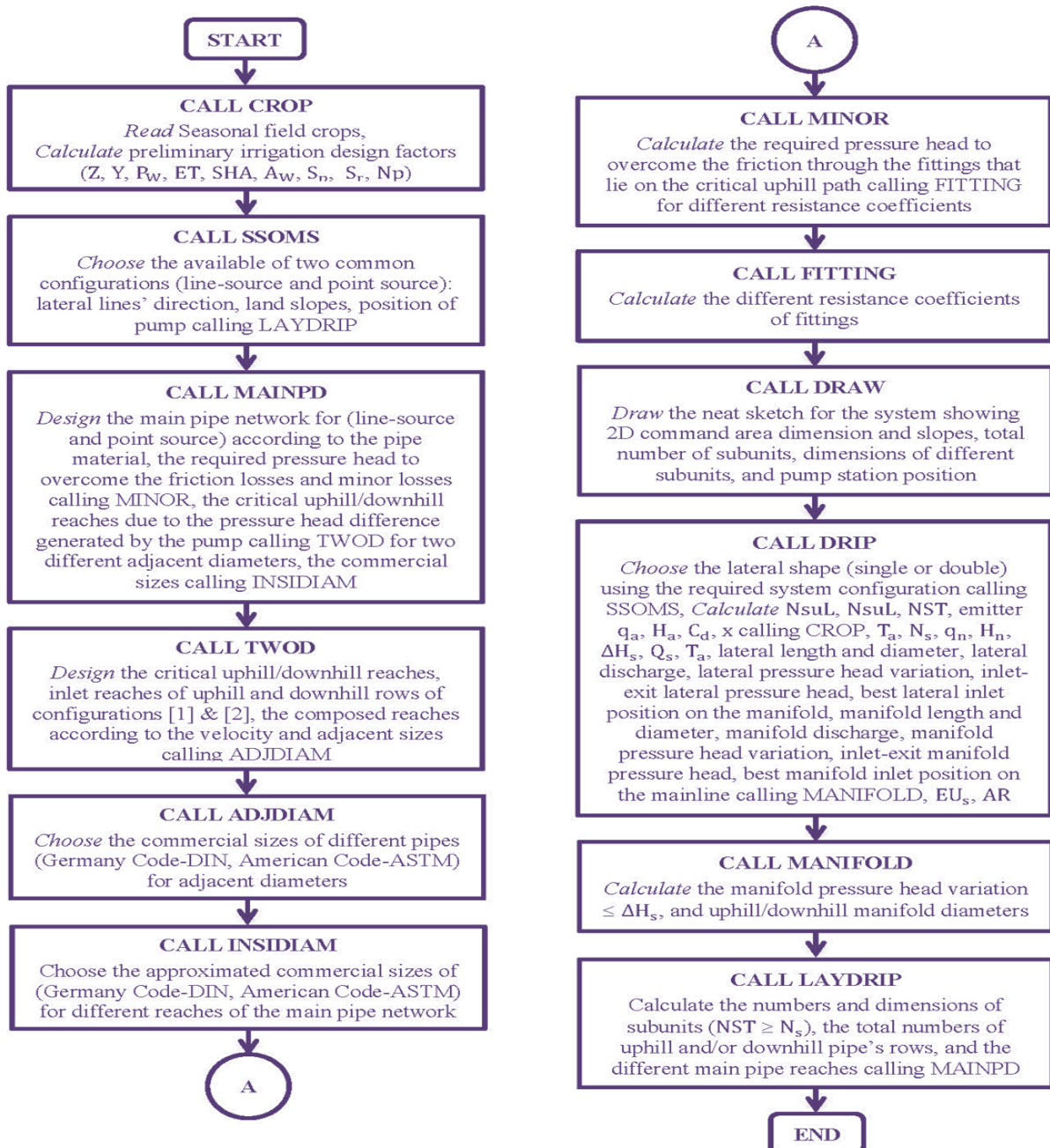
Figure 3: Flowchart of TISD program.
