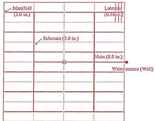
Figure 7b: Benami and Ofen design for farm layout and main pipe network (laterals are 0.58-inch PE, manifolds are IPS, and main lines are SDR 41 PVC Class 100 psi).
