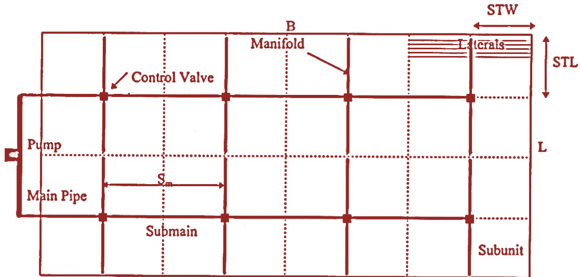
Figure 2: Configuration [2] for Trickle Irrigation Systems.
