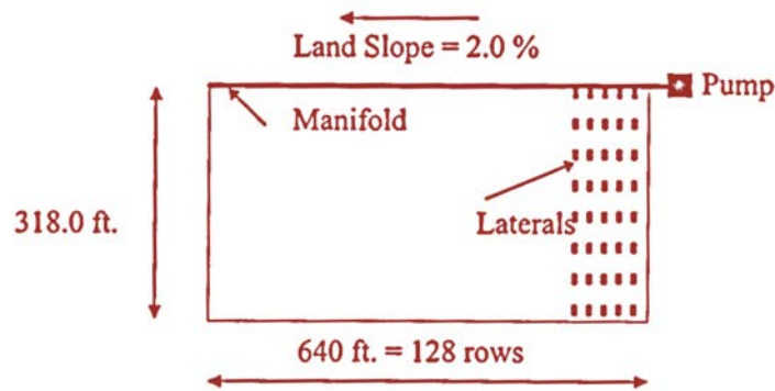
Figure 8: Model and Keller and Bliesner design for farm layout with Line-Source Drip System (Lateral lines are Single Chamber 0.625-inch (15.6 mm for model) ID-PE Tubing which discharges 26 gph/100 ft.; the manifold is buried PVC pipe).
