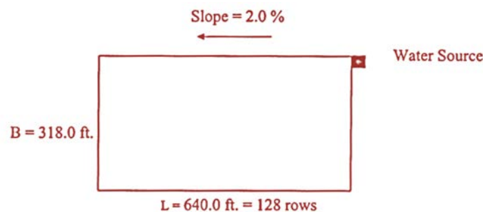
Figure 4: Tomato Field with Line-Source Drip Irrigation System [Keller and Bliesner, 1990].
