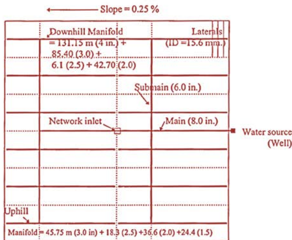
Figure 7a: Model design for farm layout and main pipe network (laterals are 18 mm PE, manifolds are SDR 26 PVC, and main lines are SDR 41 PVC).
