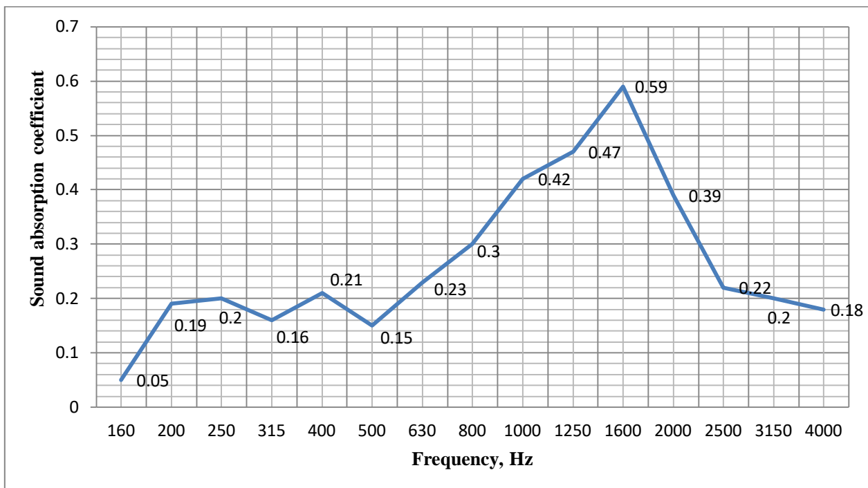
Figure 4: Dependence of the sound absorption coefficient of the cellular noise-protection panel on the sound wave frequency (sound-absorbing structure No 4 – S_f=50 \mu\text{m} , S_i = 2\text{mm} , B_p - o -shape)
