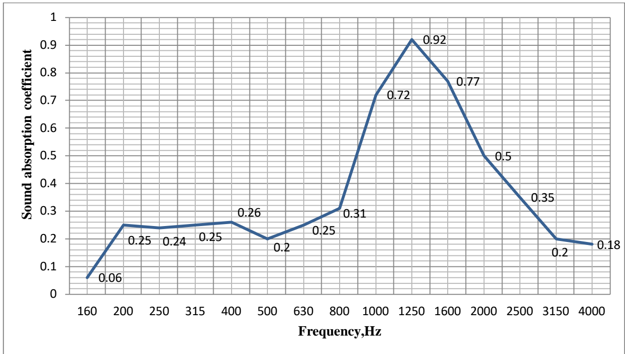
Figure 3: Dependence of the sound absorption coefficient of the cellular noise-protection panel on the sound wave frequency (sound-absorbing structure No 3, S_f=50 \mu\text{m} , S_i = 2 \text{ mm} , B_p - \Delta -shape)
