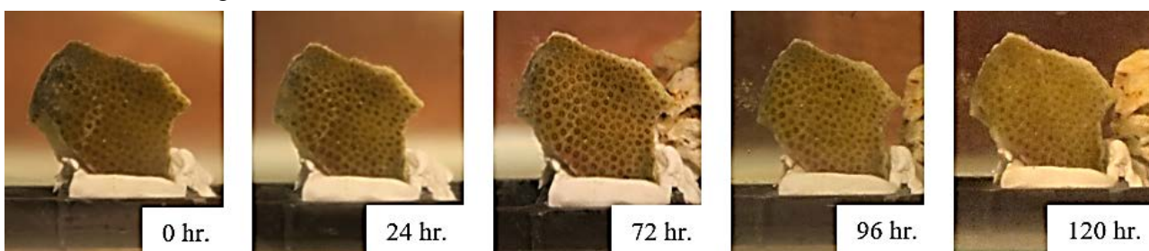
Figure 5: Change in Porites sp. at nitrate 100 µg-N/l with salinity 15 psu within 120 hrs
