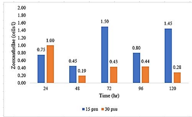
Figure 7: Zooxanthellae density at nitrate 5 µg-N/l in salinity at 15 and 30 psu
