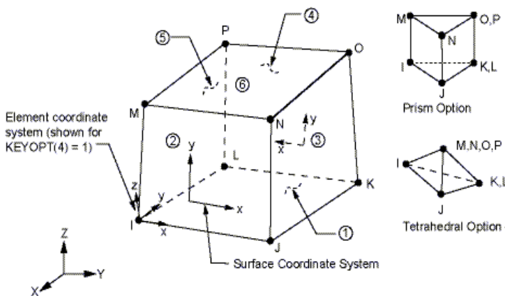
Figure 6: Solid 45 element for bearing plate
