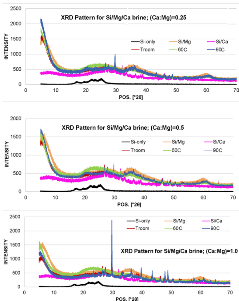
Figure 16: XRD Pattern for Si/Mg/Ca of (Ca:Mg)_0=0.25 (Top); (Ca:Mg)_0=0.5 (Middle); and (Ca:Mg)_0=1.0 (Bottom) at Various Temperatures
