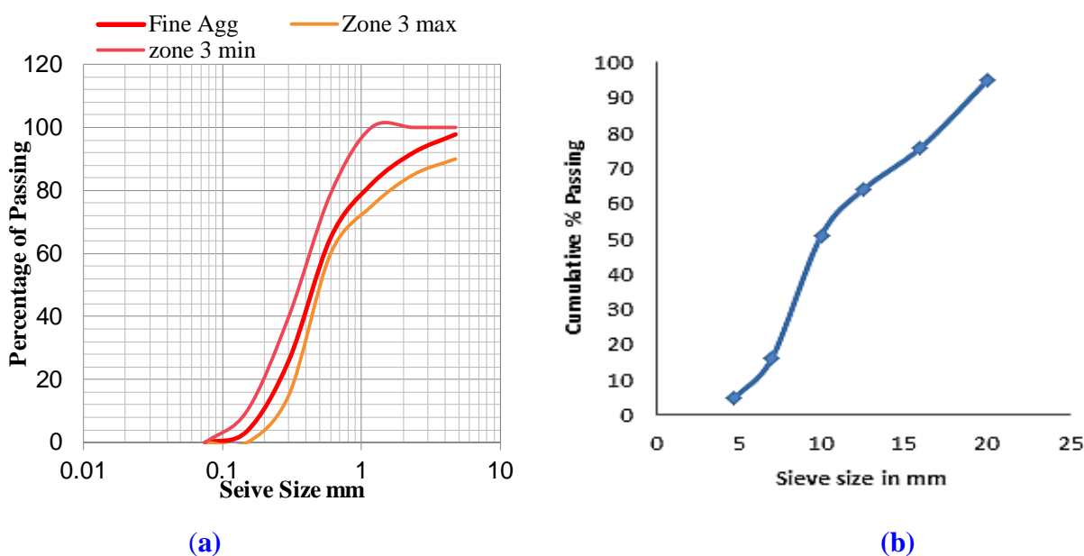
Figure 3: Gradation curve for a) Fine aggregate and b) Coarse aggregate
