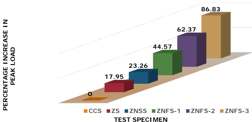
Figure 12: Effect of Steel Fibers on Deflection at Peak Load
