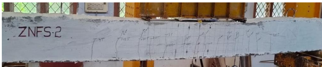
(e) Crack Pattern of ZNFS-2
