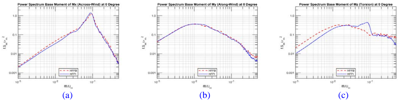
Figure 8: Power spectrum density (PSD) at 0-degree wind direction of (a) M_x (b) M_y (c) M_z
